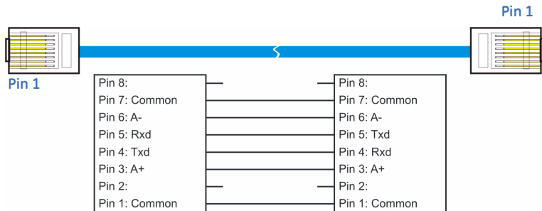
Figure 11. 4310-0034B cable
